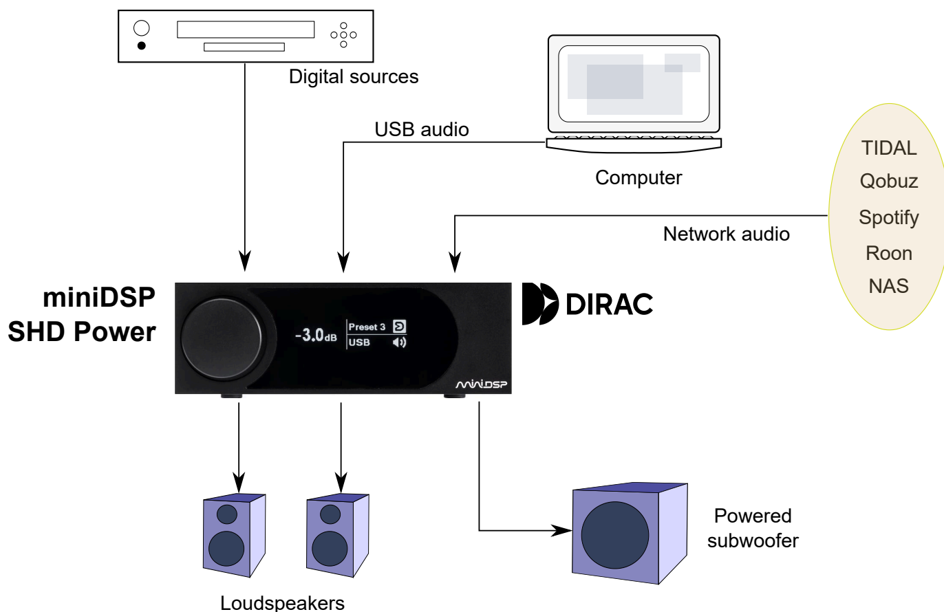
Figure 1. miniDSP SHD Power as integrated amplifier with network streaming, subwoofer integration and stereo (two-channel) Dirac Live room correction
