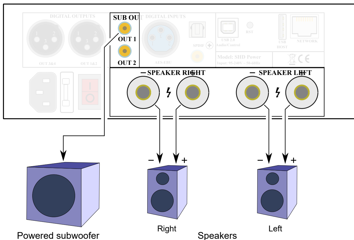
Connecting speakers and a subwoofer to the miniDSP SHD Power
