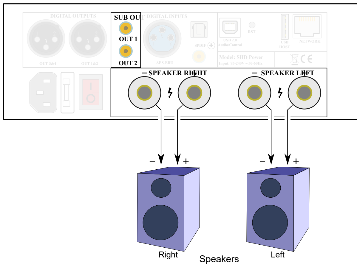
Connecting speakers to the miniDSP SHD Power
