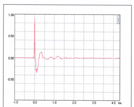
Step Response
