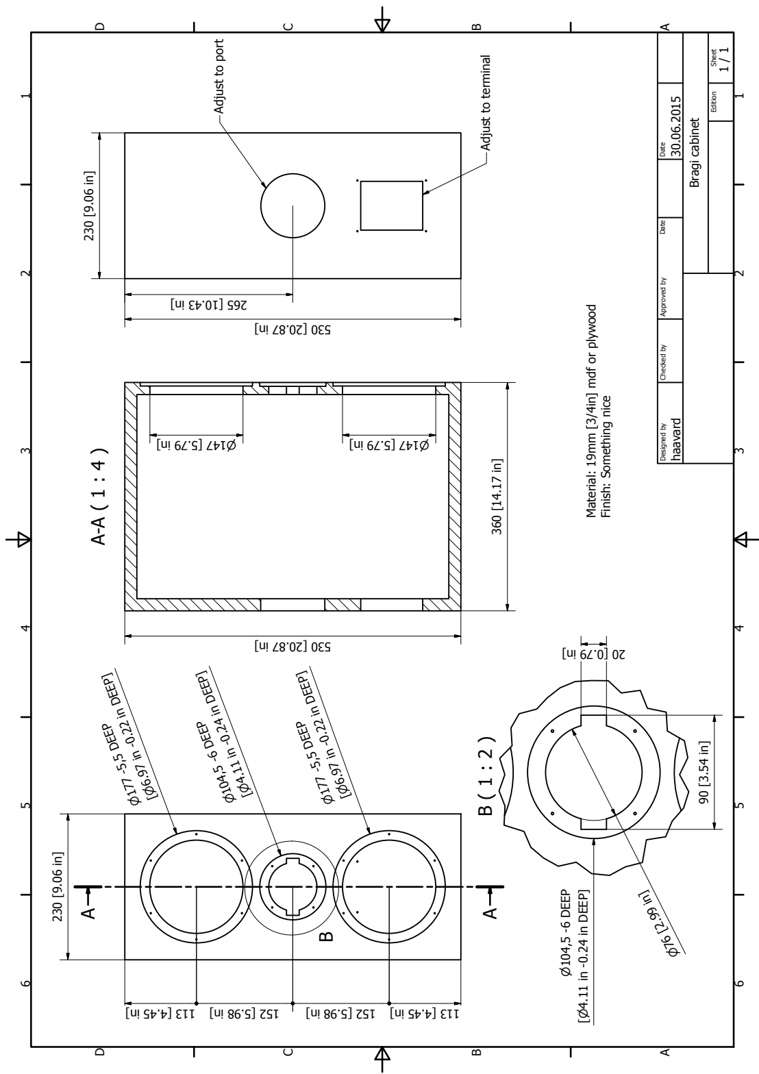
Figure 5: Cabinet drawings
