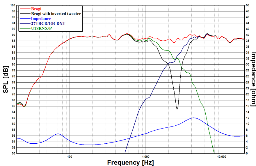
Figure 2: Anechoic free field response at 1m on tweeter axis 2.83V.
