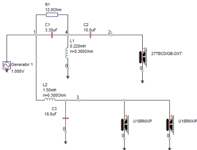
Figure 1: Crossover schematics
