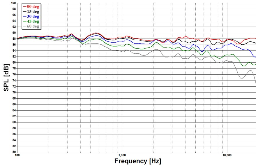
Figure 3: SPL at 1m, 2.83V, on- and off-axis
