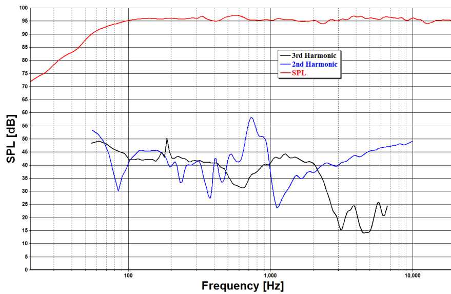
Figure 4: Harmonic distortion at 96dB SPL 1m on-axis
