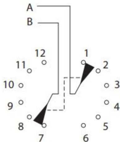
2-pole 6-way shorting rotary switch
