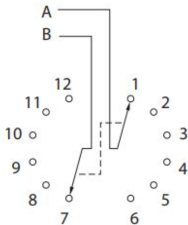
2-pole 6-way non-shorting rotary switch
