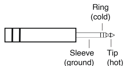
6.35mm (1/4") Phone Jack
