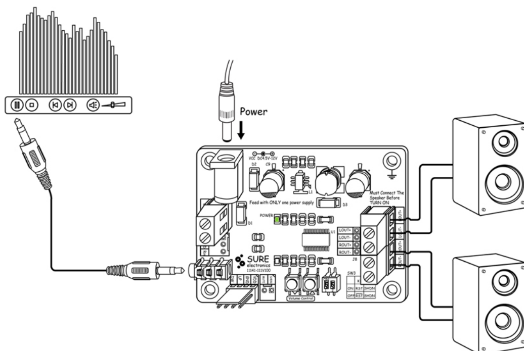
FIGURE 1-4 CONNECTION (AA-AB32131)
