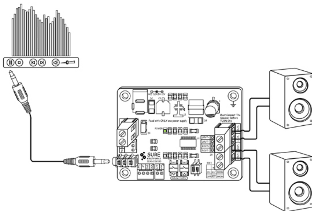
FIGURE 1-5 CONNECTION (AA-AB32133)
