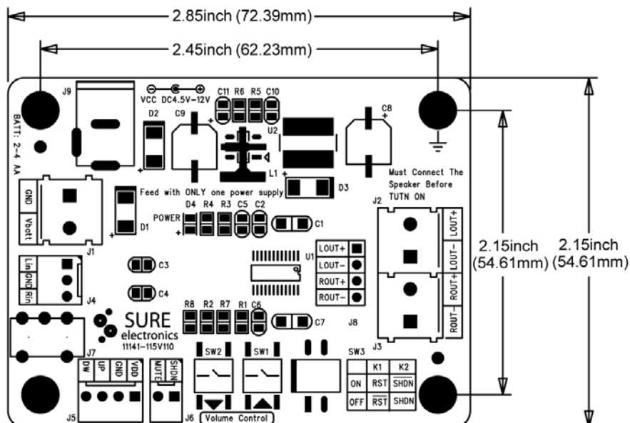
FIGURE 4-1 MECHANICAL DRAWING
