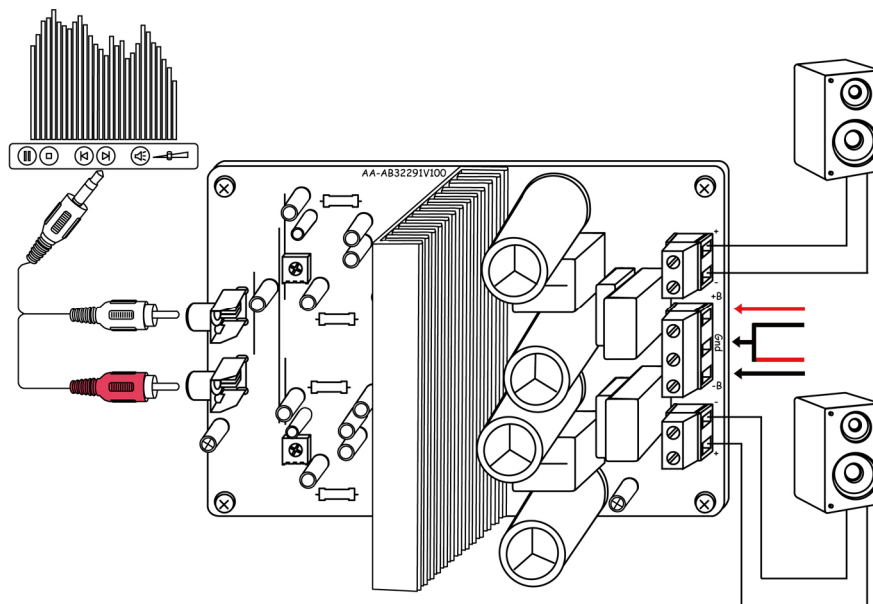
FIGURE 1-3 CONNECTION SCHEMATIC
