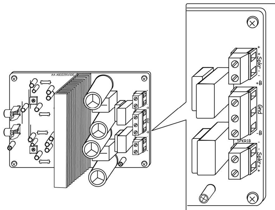
FIGURE 2-3 OUTPUT CONNECTION
