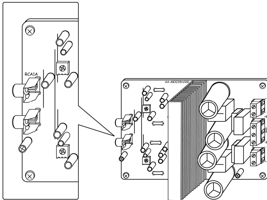
FIGURE 2-2 INPUT CONNECTION
