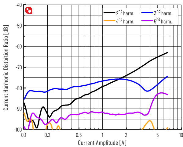
Figure 8 Current Harmonic Distortion @ 1kHz, 0-28.3Vrms
