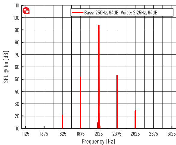
Figure 10 Intermodulation Distortion @ 250Hz 94dB, 2125Hz 94dB
