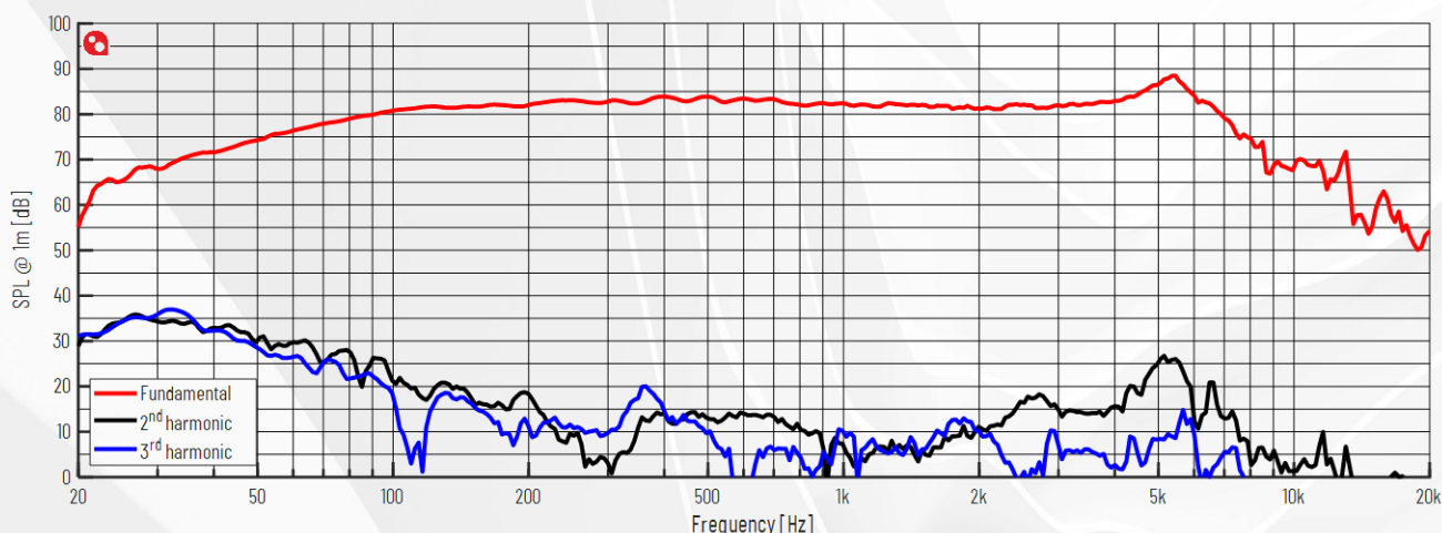
Figure 1 Frequency Response 2.83Vrms @1m
